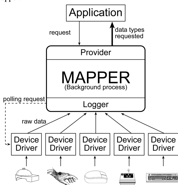
Figure 1: The Mapper provides the application with a unified view of the input devices’ capabilities
