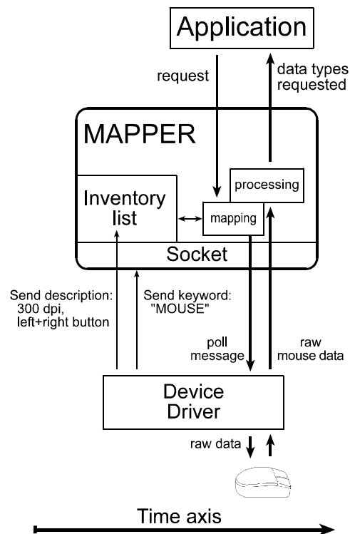
Figure 3: Example of interaction among device driver, Mapper and application requesting data
