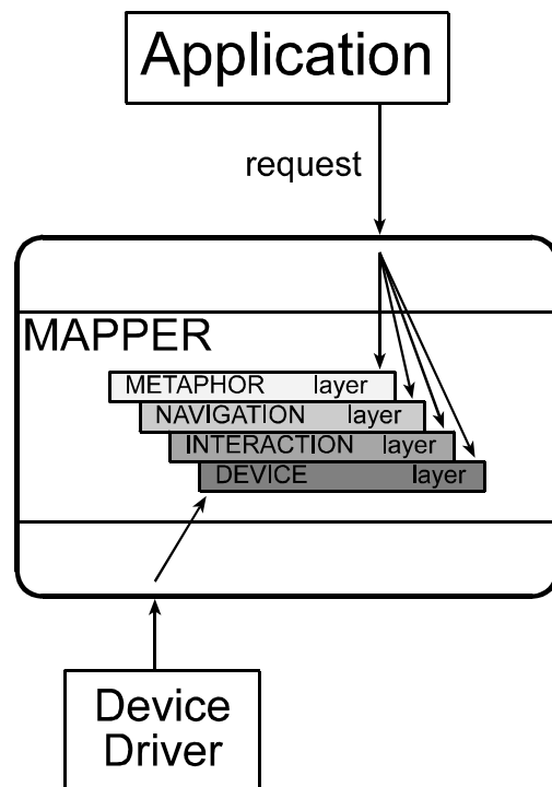
Figure 2: The application may request data on four layers of increasing abstraction
